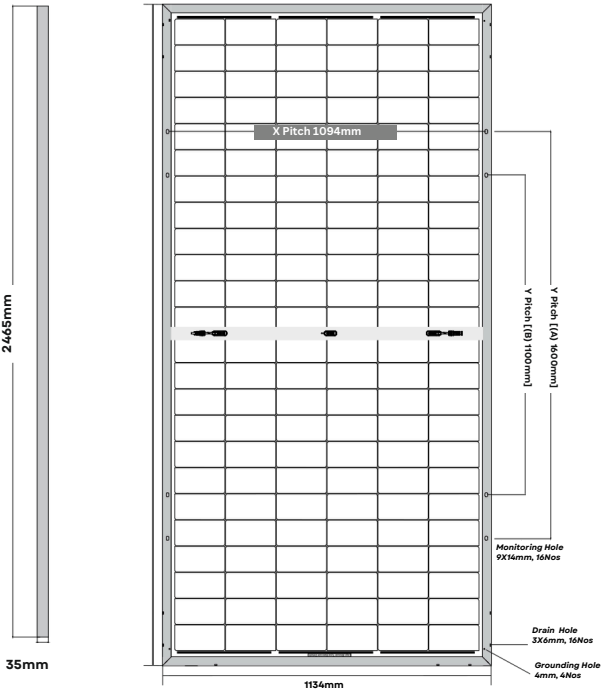
BACK VIEW
